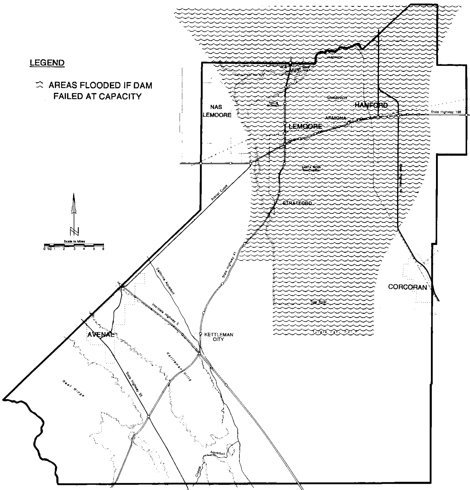
Figure 20 INUNDATION AREAS BELOW PINE FLAT DAM
