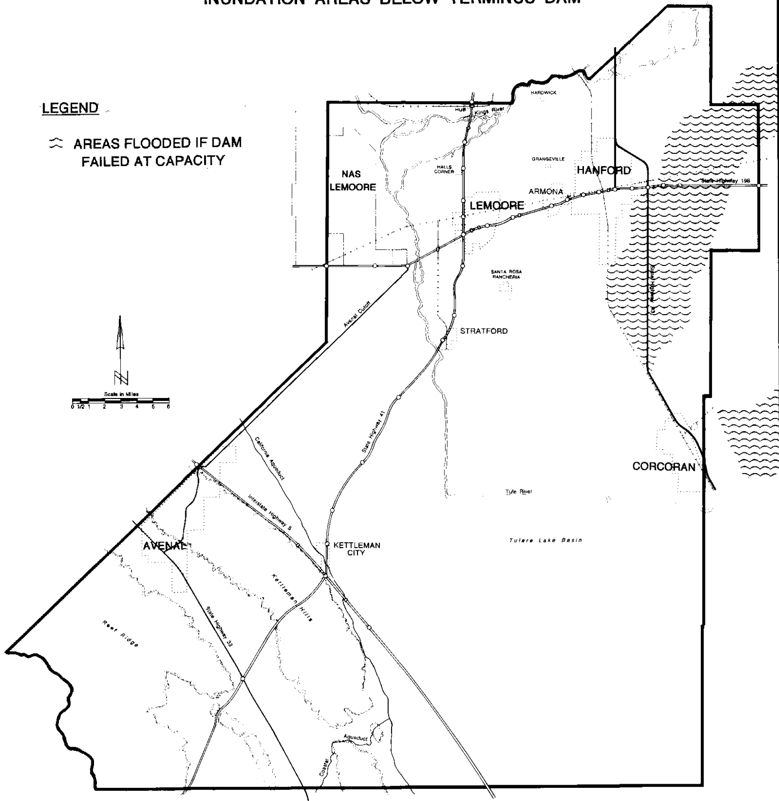
Figure 21 INUNDATION AREAS BELOW TERMINUS DAM
