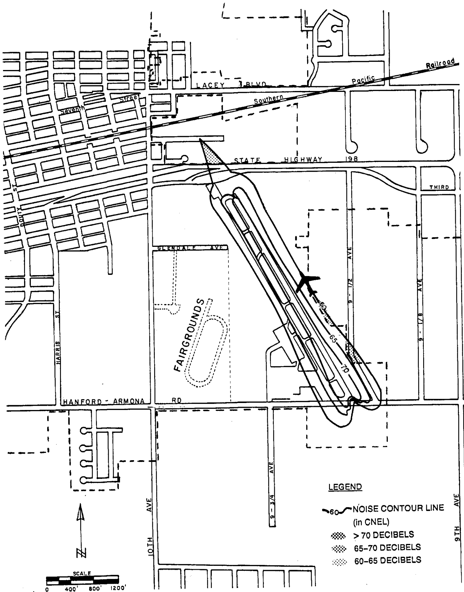
Figure 23 EXISTING HANFORD AIRPORT NOISE CONTOURS
