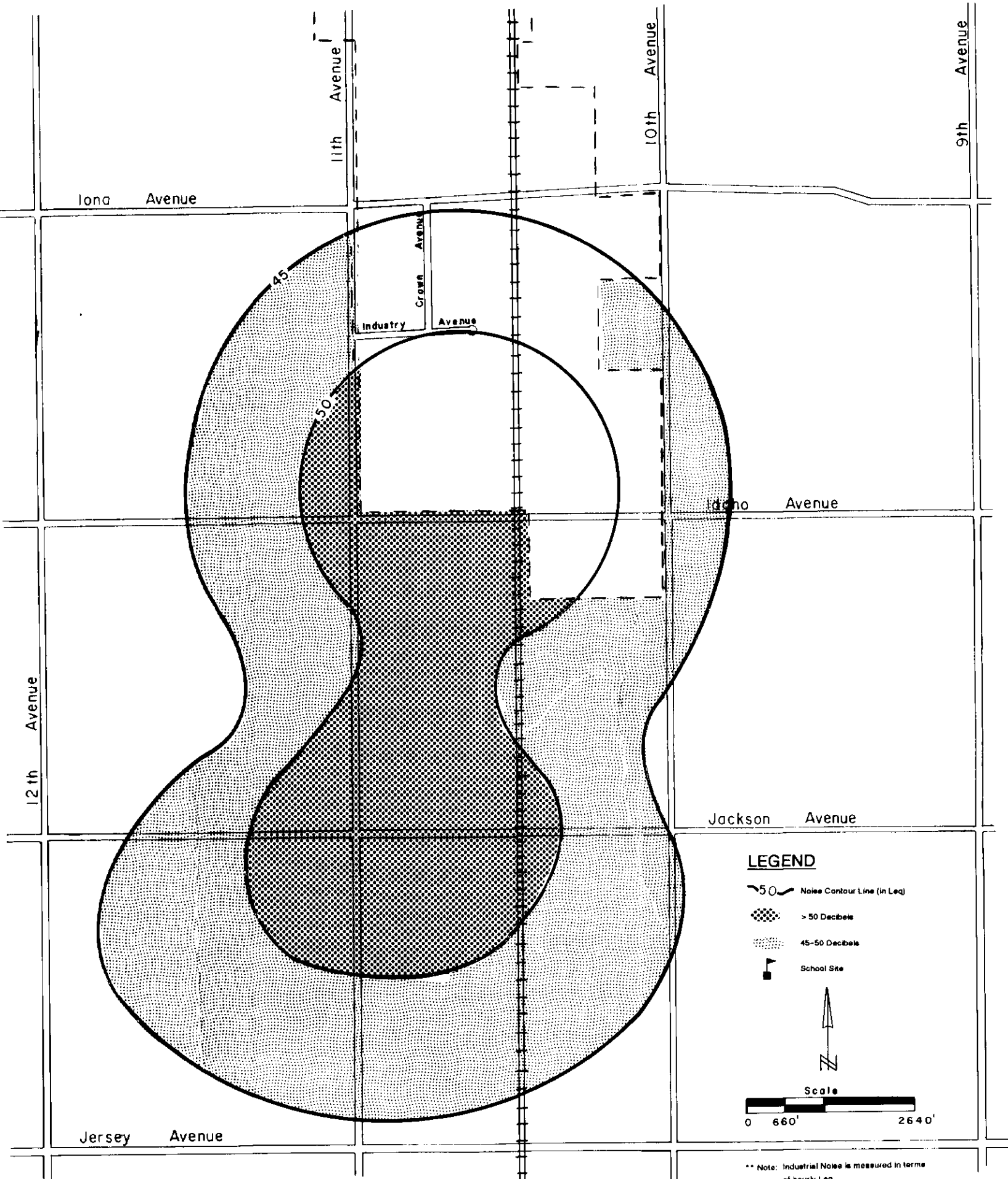
Figure 26 HANFORD INDUSTRIAL NOISE CONTOURS
