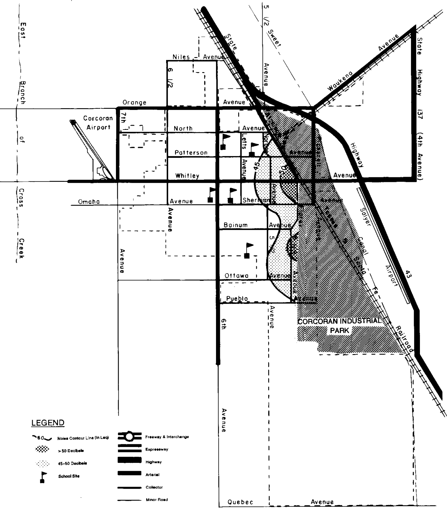
Figure 27 CORCORAN INDUSTRIAL NOISE CONTOURS
